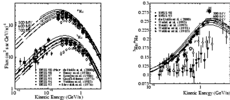
Fig. 2. Comparison of {}^4\text{He} and {}^3\text{He} BESS 98 fluxes and ratio with previous data, and with theoretical predictions of both the reacceleration model and the SLMB. The solid and dashed curves represent the reacceleration model and SLMB respectively, (top to bottom, 500, 600, 700MV).
