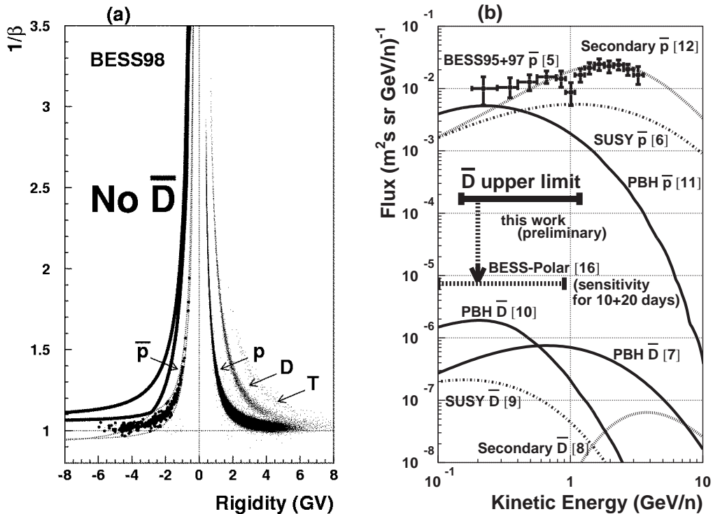
Fig. 1. (a): The identification plot of single-charge particles for '98 data. (b): Obtained upper limit on the differential cosmic-ray \bar{D} flux and the expected \bar{D} sensitivity for BESS-Polar. The calculated energy spectra of \bar{p} 's and \bar{D} 's from each origin at the solar minimum phase are also compared. The number density of PBHs in [10,11] was chosen to fit the BESS95+97 \bar{p} data using the secondary \bar{p} spectrum in [12].
